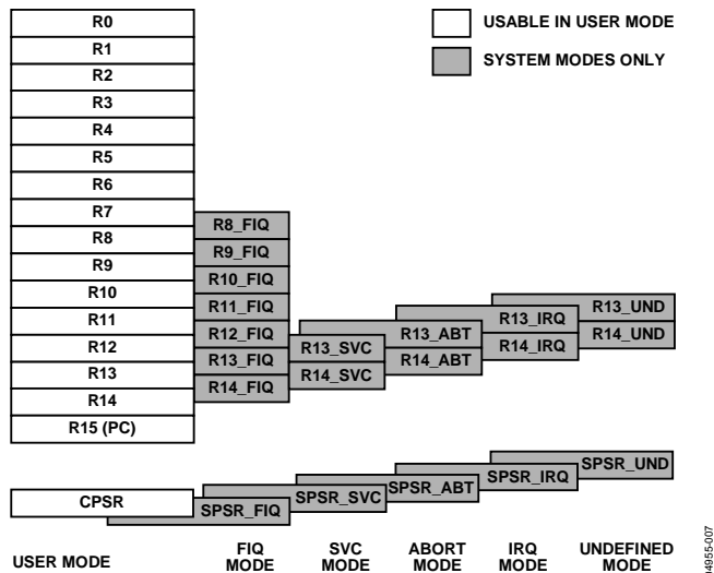
Figure 32. Register Organization
