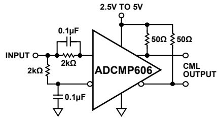
Figure 19. Self-Biased, 50% Slicer
