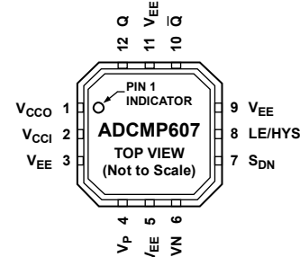
Figure 2.LFCSP Pin Configuration
