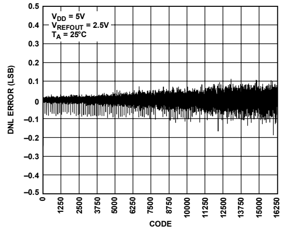
Figure 14. DNL AD5643R-5
