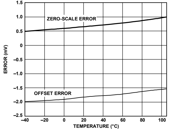
Figure 26. Zero-Scale and Offset Error vs. Temperature
