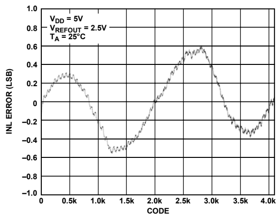
Figure 12. INL AD5623R-5
