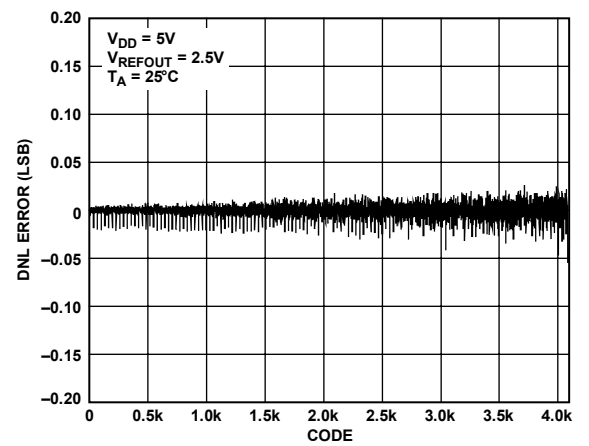
Figure 15. DNL AD5623R-5
