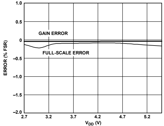
Figure 27. Gain Error and Full-Scale Error vs. Supply
