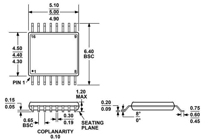
Figure 59. 16-Lead Thin Shrink Small Outline Package [TSSOP] (RU-16) Dimensions shown in millimeters
