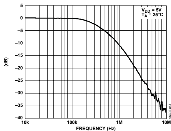
Figure 50. Multiplying Bandwidth
