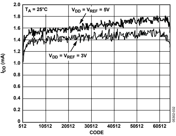
Figure 32. Supply Current vs. Code
