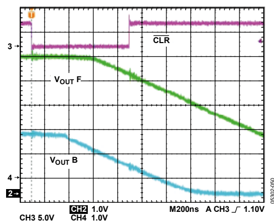
Figure 49. Hardware \overline{CLR}
