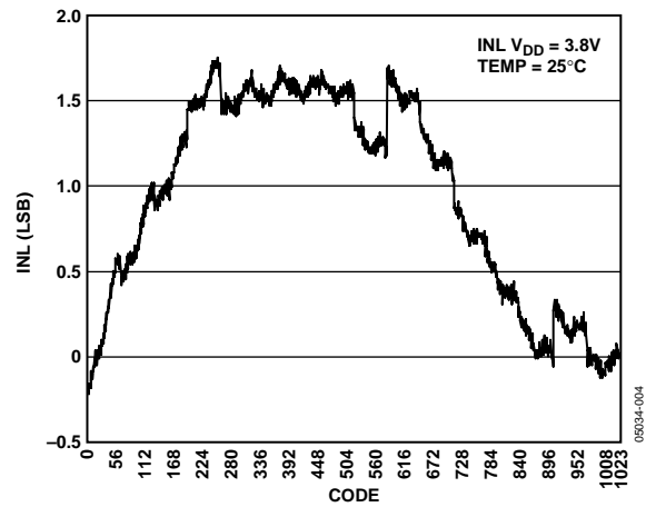
Figure 6. Typical INL Plot
