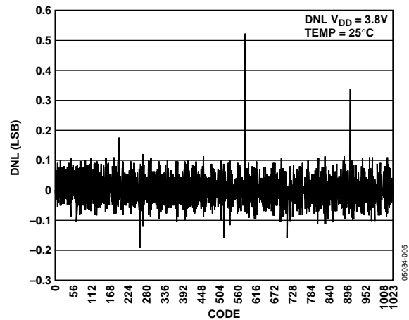
Figure 7. Typical DNL Plot
