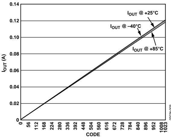
Figure 11. Sink Current vs. Code vs. Temperature ( V_{DD} = 3.6\text{ V} )
