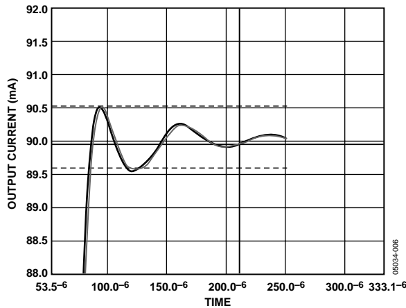
Figure 8. \frac{1}{4} to \frac{3}{4} Scale Settling Time ( V_{DD} = 3.6\text{ V} )
