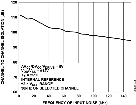
Figure 22. Channel-to-Channel Isolation
