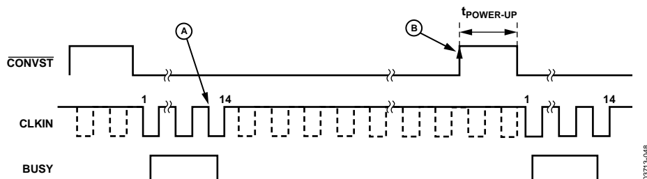
Figure 38. Autoshutdown/Autostandby Mode
