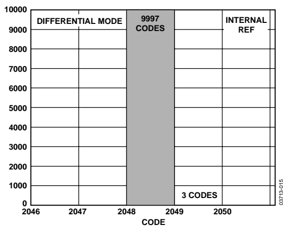
Figure 12. AD7934 Histogram of Codes for 10k Samples @ V_{DD} = 5\text{ V} with the Internal Reference
