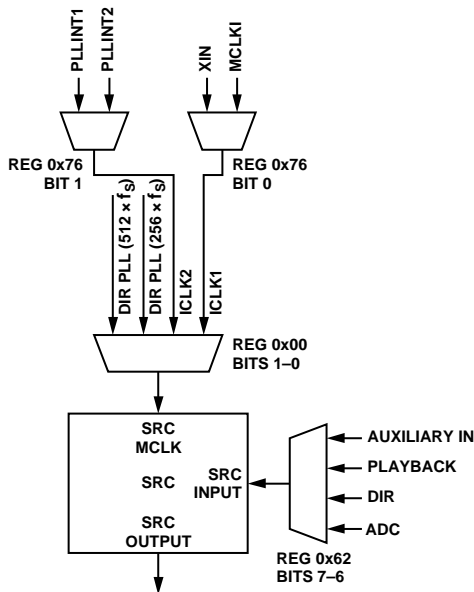
Figure 33. Clock and Datapath Control on the SCR
