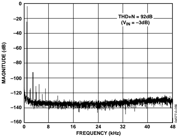
Figure 22. ADC THD + N, f_s = 96 \text{ kHz}
