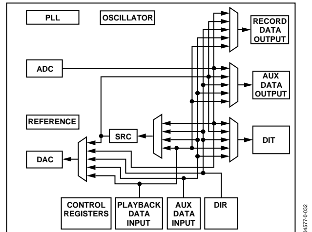
Figure 52. Datapath
