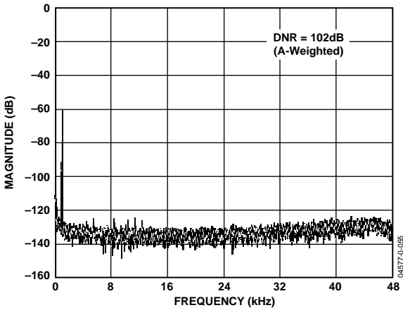
Figure 21. ADC Dynamic Range, f_s = 96 \text{ kHz}
