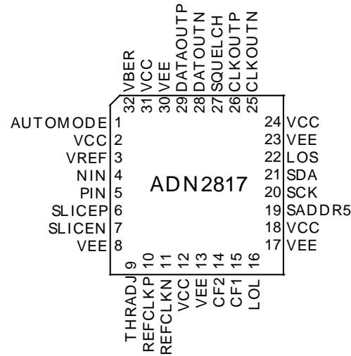
Figure 4. Pin Configuration
