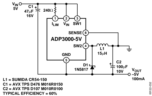
Figure 33. 5 V to -5 V/100 mA Inverter
