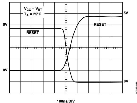
Figure 9. \overline{\text{RESET}} , RESET Assertion
