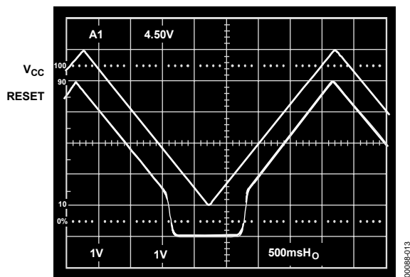
Figure 6. ADM707/ADM708 RESET Output Voltage vs. Supply Voltage
