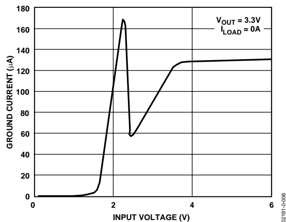
Figure 6. Ground Current vs. Supply Voltage
