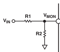
Figure 11. Scaling V_{MON} to a Higher Reset Voltage
