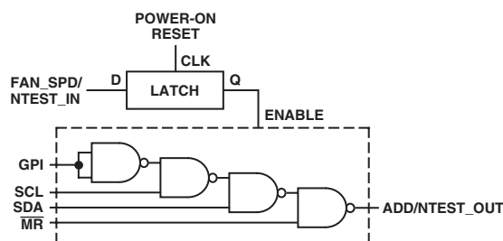
Figure 12. NAND Tree
