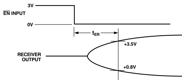
Figure 13. Receiver Disable Timing
