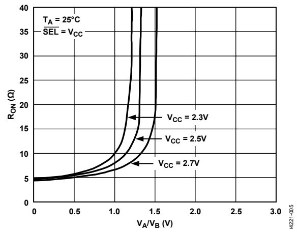
Figure 5. On Resistance vs. Input Voltage
