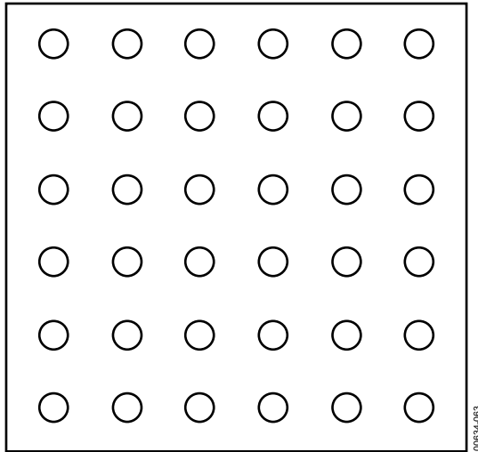
Figure 63. Proposed Via Pattern
