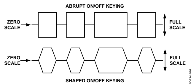
Figure 46. Shaped On/Off Keying
