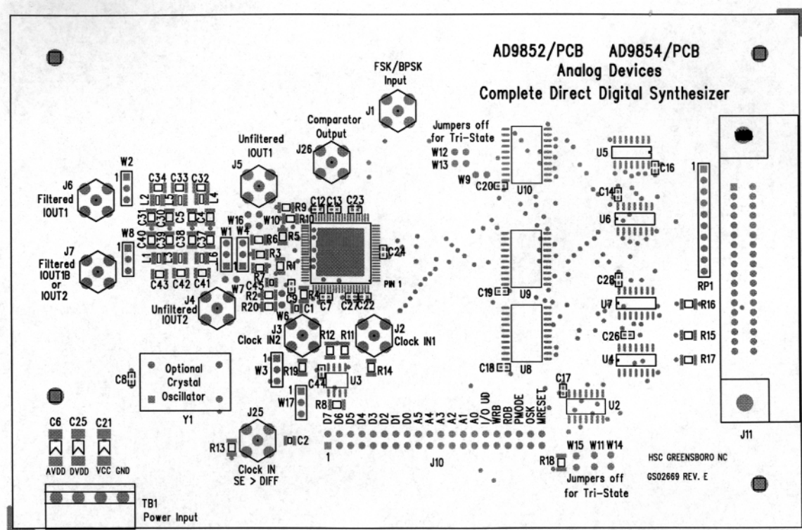
Figure 67. Assembly Drawing
