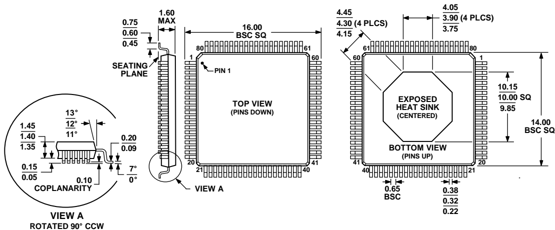
Figure 72. 80-Lead Low Profile Quad Flat Package, Edquad [LQFP_ED] (SQ-80-2)
