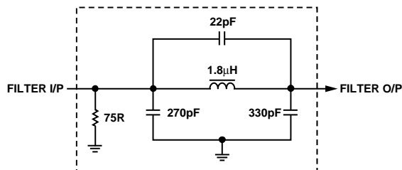
Figure 79. Output Filter
