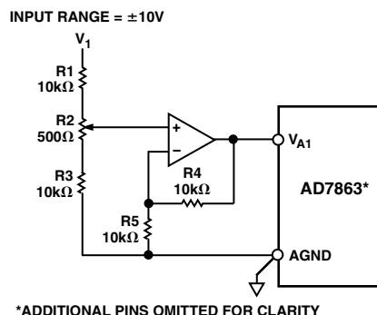
Figure 4. Full-Scale Adjust Circuit
