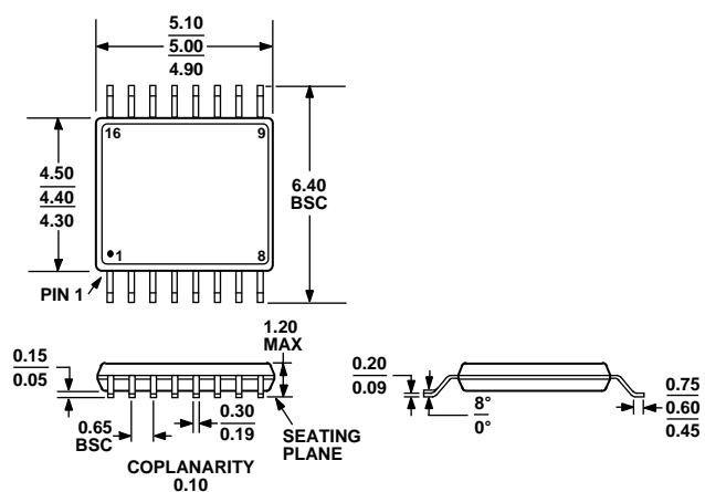
Figure 66. 16-Lead Thin Shrink Small Outline Package (TSSOP) (RU-16) Dimensions shown in millimeters
