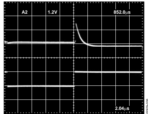
Figure 26. Midscale Glitch Energy Code 0x80 to 0x7F
