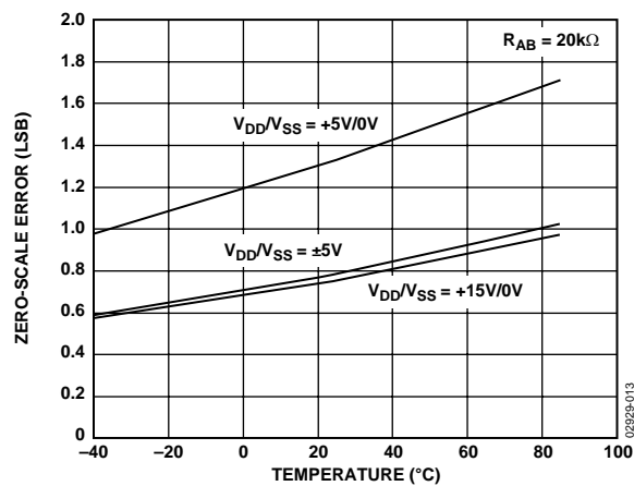
Figure 13. Zero-Scale Error
