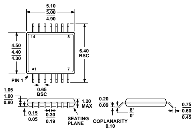
Figure 65. 14-Lead Thin Shrink Small Outline Package (TSSOP) (RU-14) Dimensions shown in millimeters
