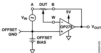
Figure 35. Inverting Gain
