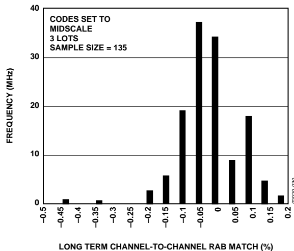
LONG TERM CHANNEL-TO-CHANNEL R AB MATCH (%) Figure 30. Channel-to-Channel Resistance Matching (AD5282)
