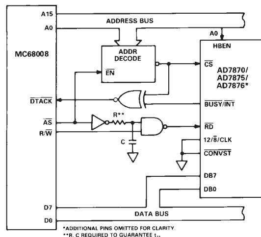
Figure 20. MC68008 Byte Interface
