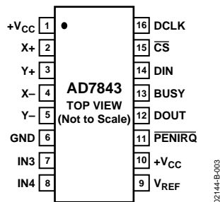
Figure 3. Pin Configuration QSOPT/TSSOP
