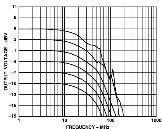
TPC 18. Output Voltage vs. Frequency; V_S = \pm 6 V, R_L = 100 \Omega ; G = +5
