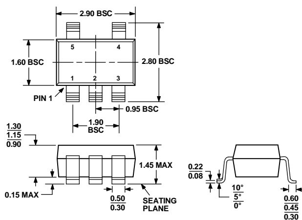
Dimensions shown in millimeters and (inches)
