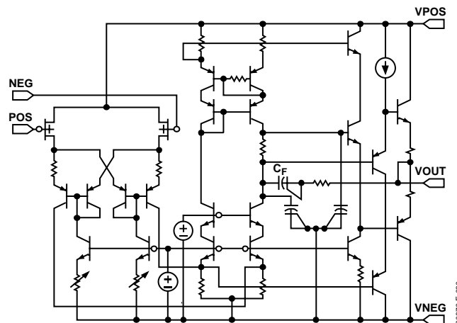
Figure 32. Simplified Schematic
