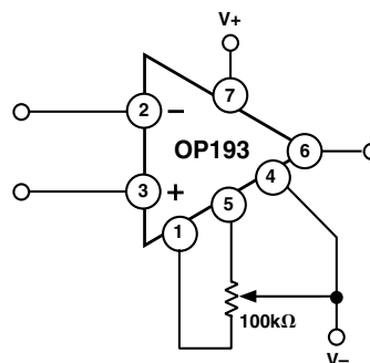
Figure 4. Offset Nulling Circuit
