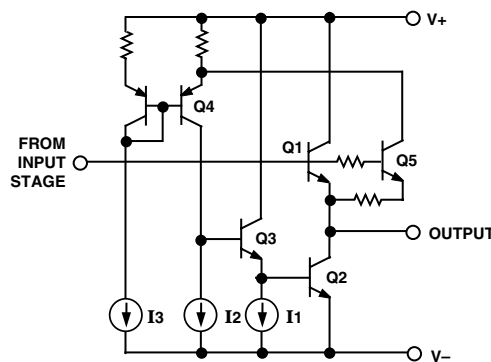
Figure 2. OP193/OP293/OP493 Equivalent Output Circuit
