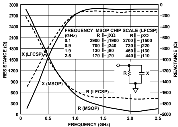
Figure 11. Input Impedance
