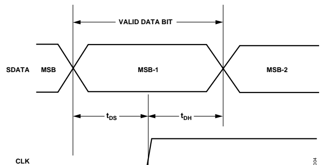
Figure 4. SDATA Timing
