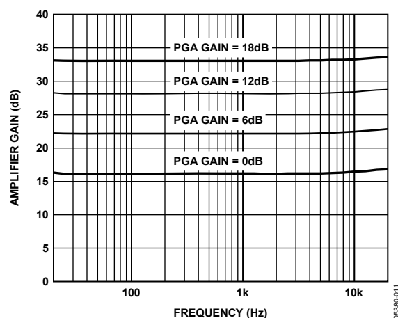
Figure 11. Amplifier Gain vs. Frequency, 6 \Omega Load, PVDD = 12 V
