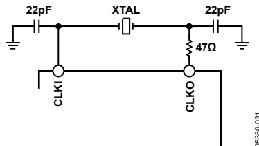
Figure 25. Crystal Connection
