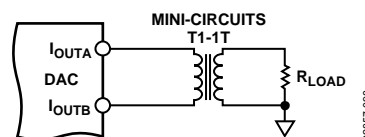
Figure 98. Transformer-Coupled Output Circuit
