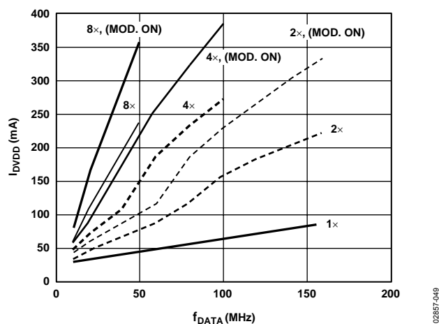
Figure 49. I_{DVDD} VS. f_{DATA} VS. Interpolation Rate, PLL Disabled
