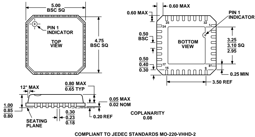
Figure 57. 32-Lead Lead Frame Chip Scale Package [LFCSP] 5 mm x 5 mm Body (CP-32-2) Dimensions shown in millimeters
