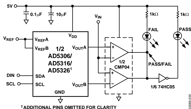
Figure 39. Window Detection
