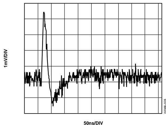
Figure 28. DAC-to-DAC Crosstalk
