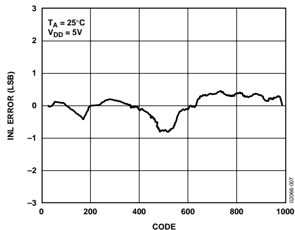
Figure 7. AD5316 INL
