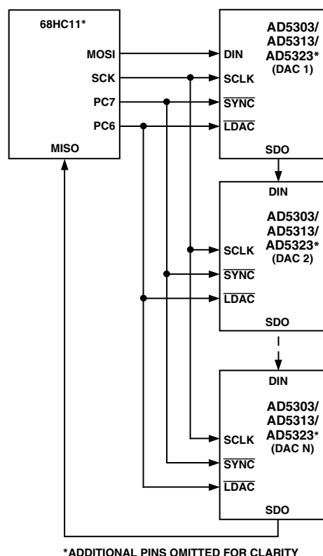
Figure 22. Daisy-Chain Mode
