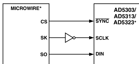
Figure 14. AD5303/AD5313/AD5323 to MICROWIRE Interface
