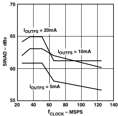
TPC 10. SINAD vs. f_{\text{CLK}} and I_{\text{OUTFS}} @ f_{\text{OUT}} = 5 \text{ MHz} and 0 \text{ dBFS}
