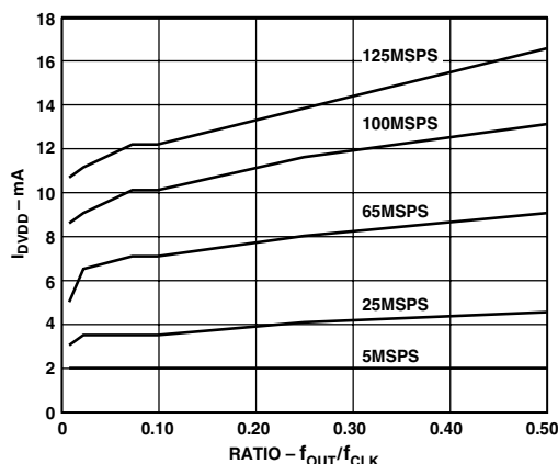
Figure 15. I_{DVDD} vs. Ratio @ DVDD = 3\text{ V}
