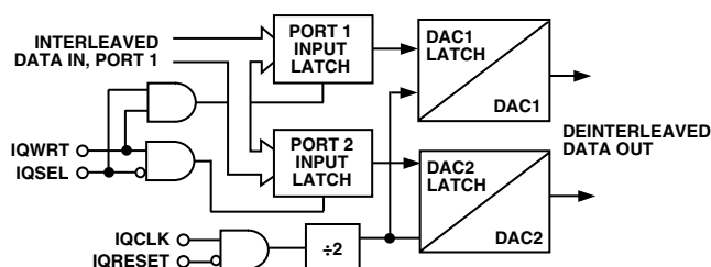
Figure 8. Latch Structure Interleaved Mode
