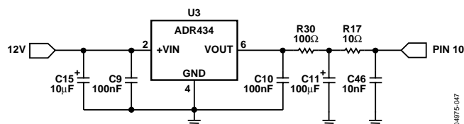
Figure 45. Reference Connection
