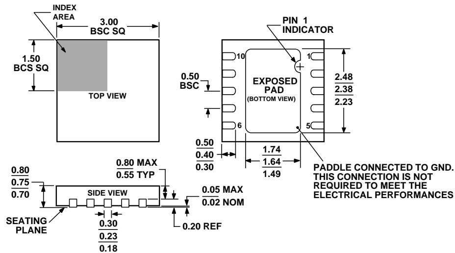
Figure 49. 10-Lead Lead Frame Chip Scale Package [QFN¹ (LFCSP_WD)] 3 mm × 3 mm Body, Very Very Thin, Dual Lead (CP-10-9)
