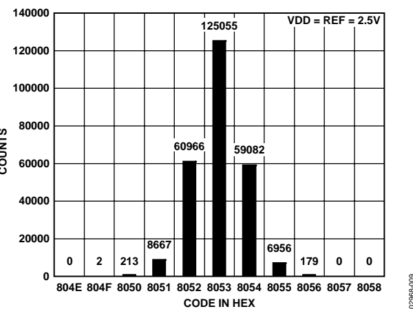
Figure 10. Histogram of a DC Input at the Code Center
