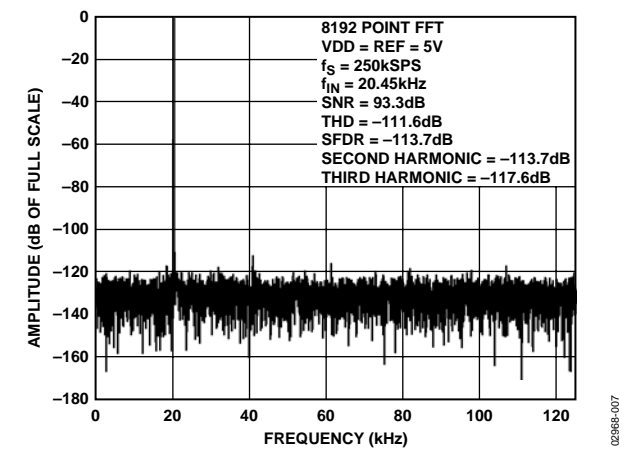
Figure 8. FFT Plot
