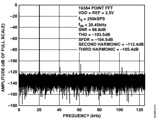
Figure 11. FFT Plot
