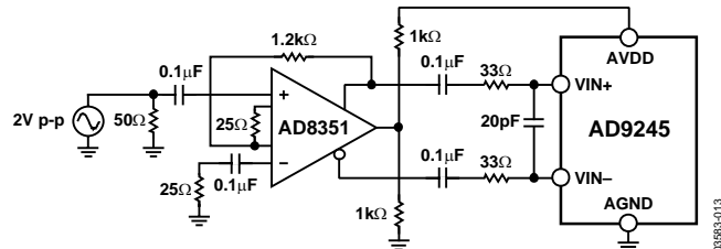
Figure 40. Differential Input Configuration Using the AD8351
