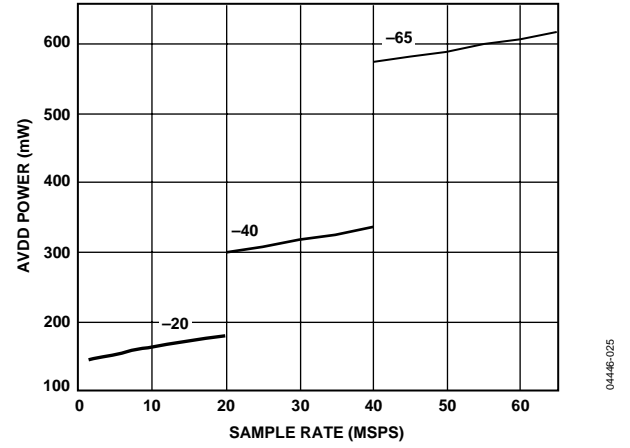
Figure 25. Analog Power Consumption vs. FS
