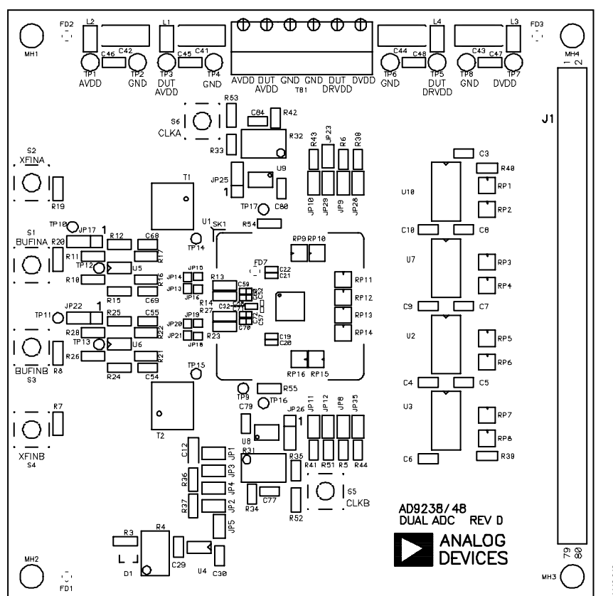
Figure 47. PCB Top Silkscreen (Note that the PCB Supports Both the AD9238 and AD9248 LQFP)
