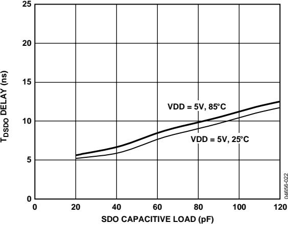
Figure 22. t_{\text{DSO}} Delay vs. Capacitance Load and Supply
