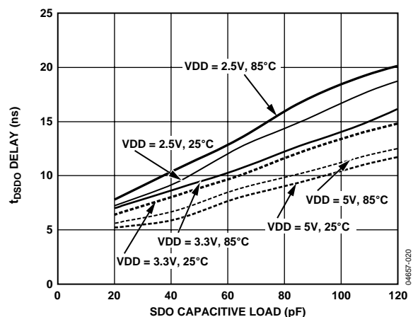
Figure 20. t_{DSO} vs. Capacitance Load and Supply
