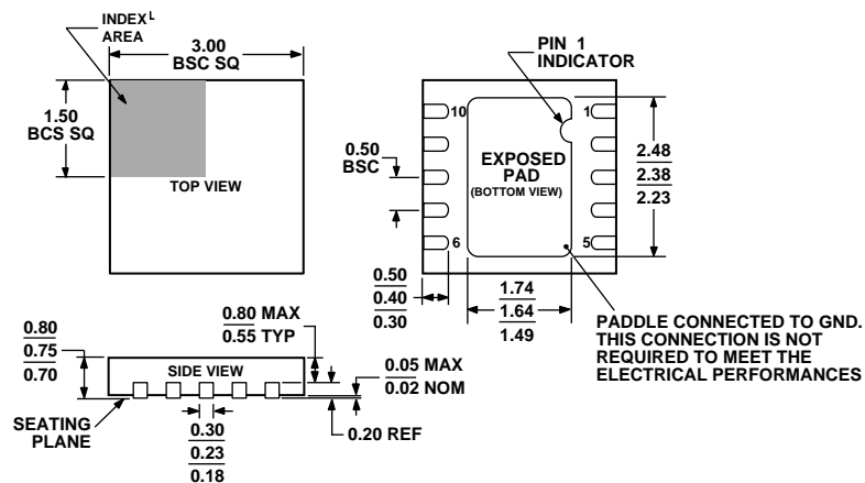
Figure 45. 10-Lead Lead Frame Chip Scale Package [QFN 1 (LFCSP)] 3 mm × 3 mm Body (CP-10)
