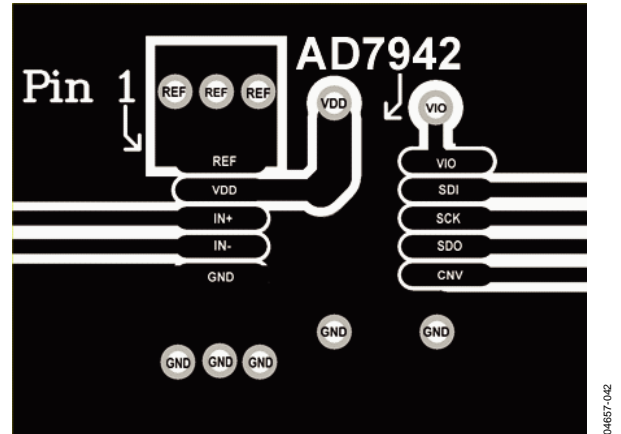
Figure 42. Example of Layout of the AD7942 (Top Layer)
