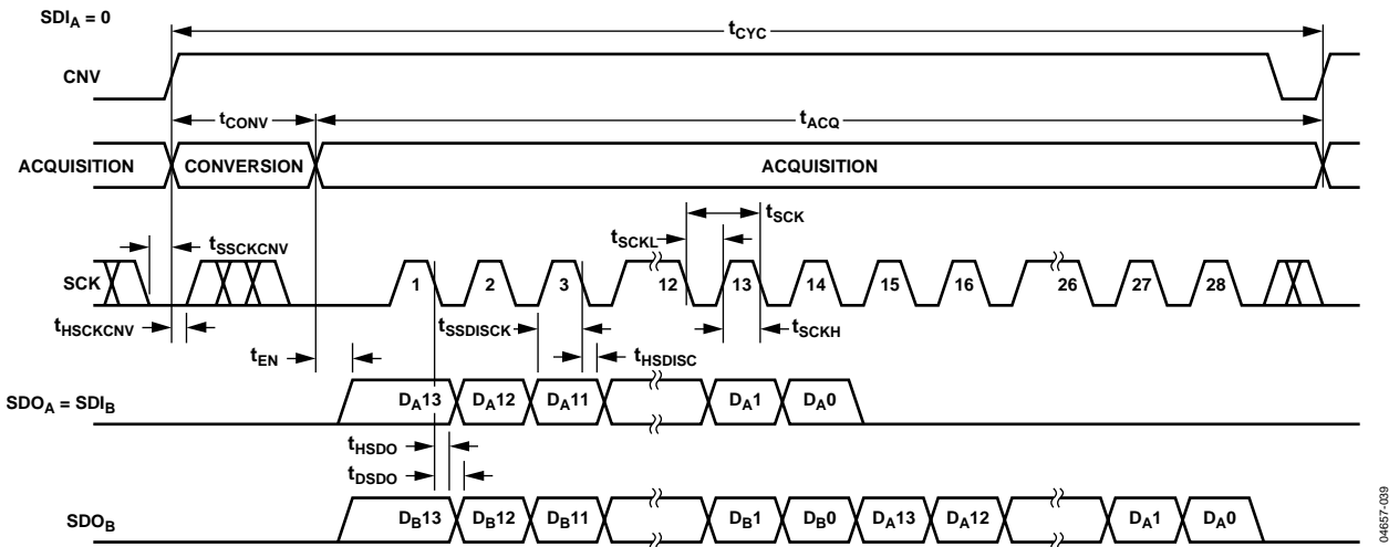
Figure 39. Chain Mode, No Busy Indicator, Serial Interface Timing
