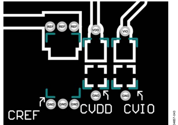
Figure 43. Example of Layout of the AD7942 (Bottom Layer)
