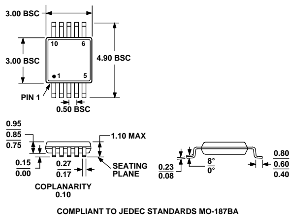
Figure 44. 10-Lead Mini Small Outline Package [MSOP] (RM-10)
