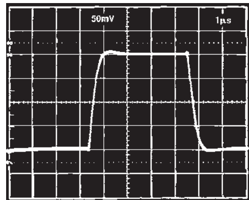
TPC 26. Unity-Gain Inverter Small Signal Pulse Response
