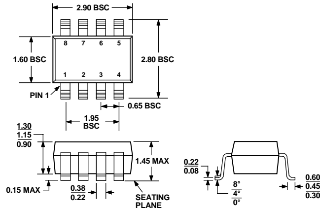
Figure 43. 8-Lead Small Outline Transistor Package [SOT-23] (RT-8) Dimensions shown in millimeters
