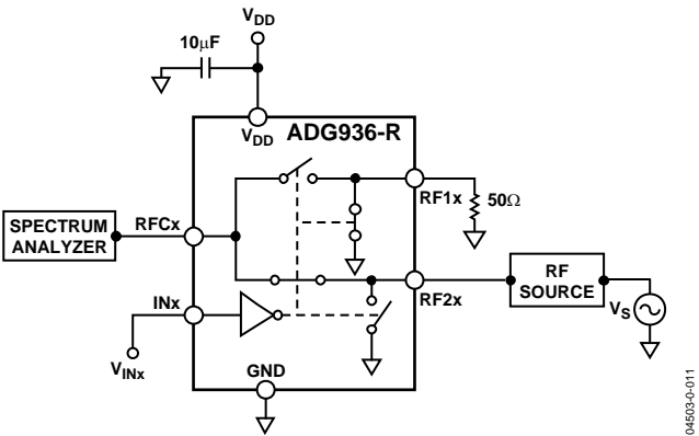
Figure 26. P_{-1dB}
