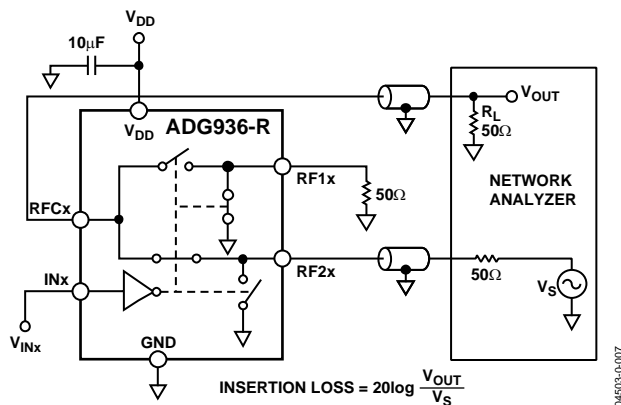
Figure 22. Insertion Loss
