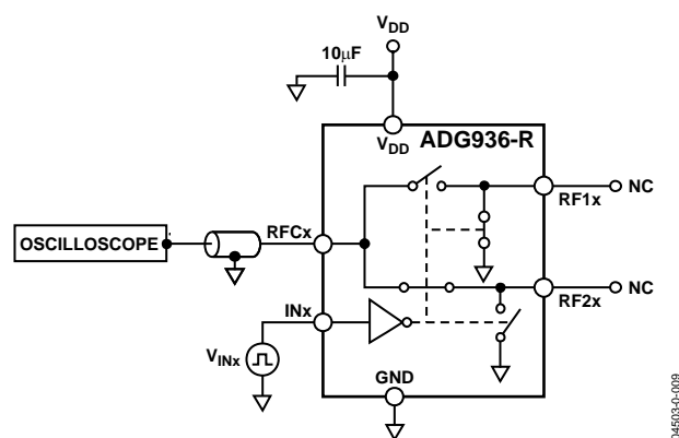
Figure 24. Video Feedthrough
