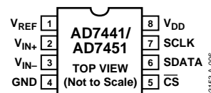
Figure 6. 8-Lead MSOP
