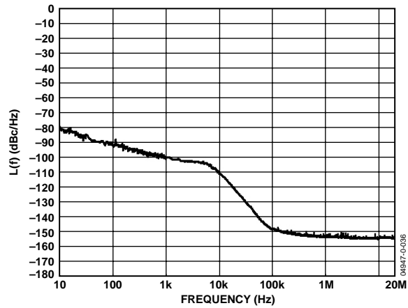
Figure 29. Total System Phase Noise for 105 MHz Converter Clock
