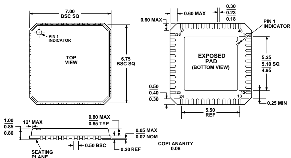
Figure 42. 48-Lead Lead Frame Chip Scale [LFCSP]
