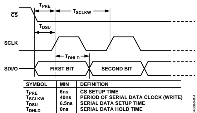
Figure 40. Timing Diagram for Data Write to AD9540
