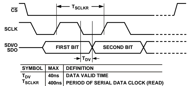
Figure 41. Timing Diagram for Data Read to AD9540
