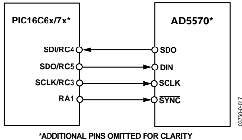
Figure 44. AD5570 to PIC16C6x/7x Interface
