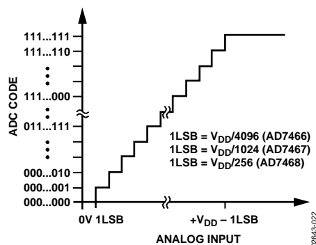
Figure 22. AD7466/AD7467/AD7468 Transfer Characteristics
