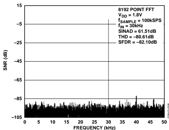
Figure 8. AD7467 Dynamic Performance at 100 kSPS
