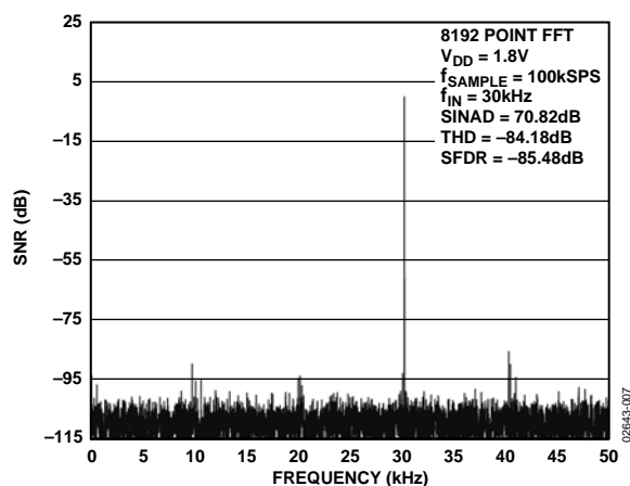
Figure 7. AD7466 Dynamic Performance at 100 kSPS
