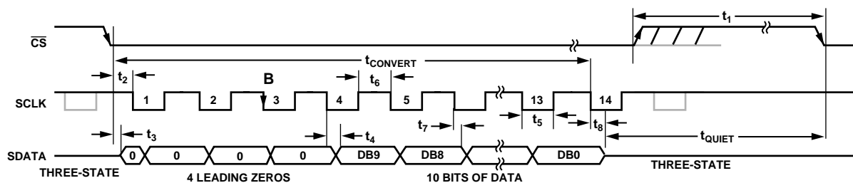
Figure 31. AD7467 Serial Interface Timing Diagram
