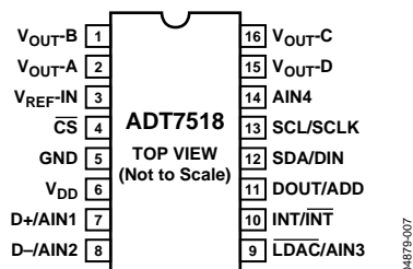
Figure 7. Pin Configuration QSO8
