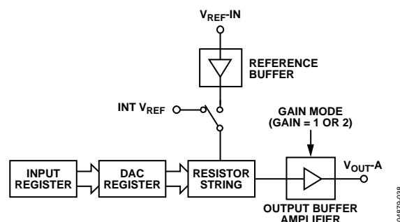
Figure 38. Single DAC Channel Architecture
