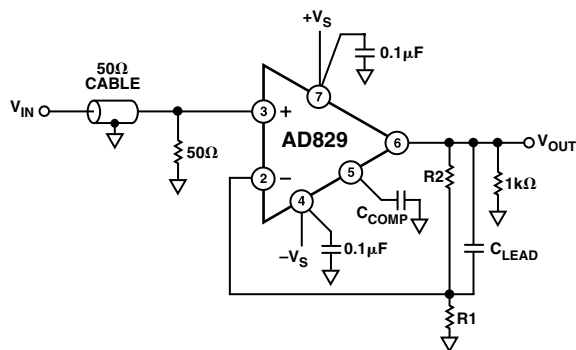
Figure 27. Noninverting Amplifier Connection Using External Shunt Compensation
