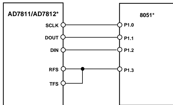
Figure 22. Interfacing to the 8051 Using I/O Ports
